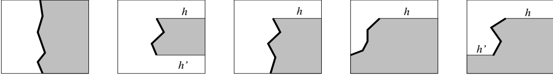
Figure 7: The boxes represent \Delta_i and \vec{d}_b is the rightward direction. The shaded areas represent the projected lower blue curtains. The bold chains are the p-tails. h and h' are the p-fingeredges. In the first four figures, the p-tails are also the extended p-tails. In the last figure, h' and the p-tail form the extended p-tail.
