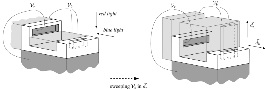
Figure 3: An object \mathcal{Q} and its shadow volume. \mathcal{V}_r intersects two connected components of \mathcal{B} \setminus (\mathcal{V}_b^* \cup \mathcal{Q}) .
