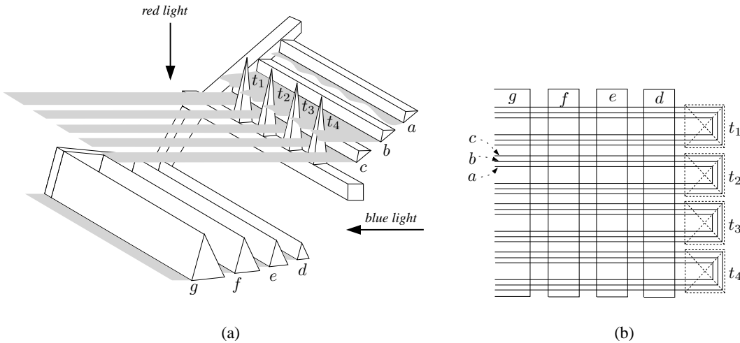
Figure 4: \Theta(n^3) complexity.
