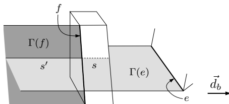
Figure 5: A finger edge consisting of two segments: s lying on a facet parallel to \vec{d}_b , and s' lying on \Gamma(f) .
