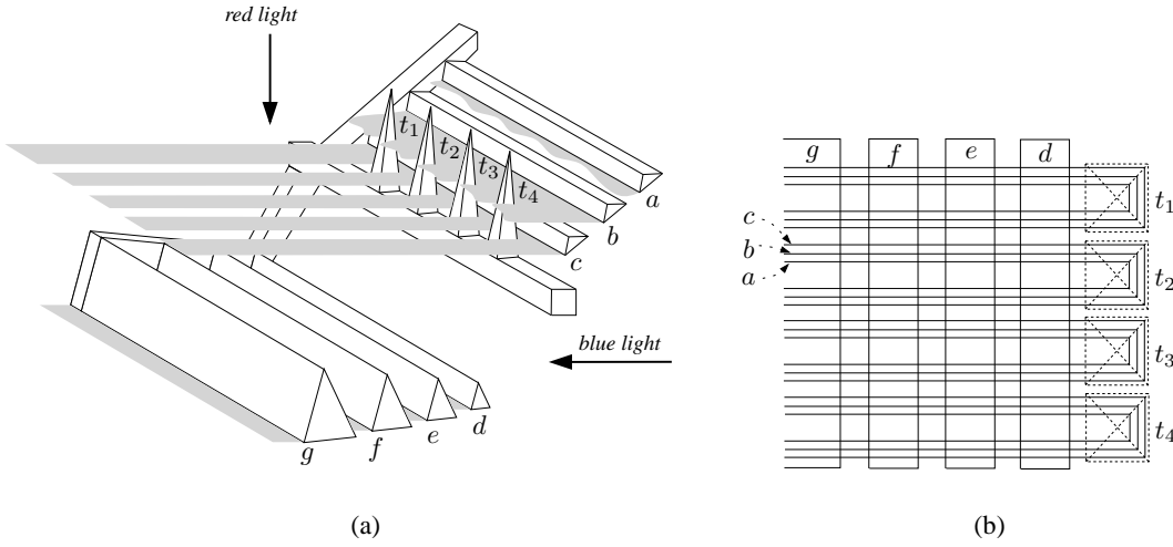
Figure 4: \Theta(n^3) complexity.
