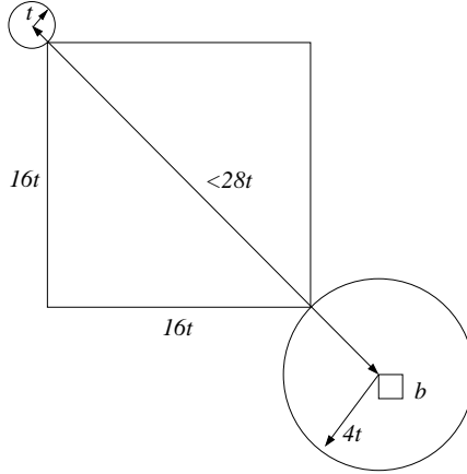
Figure 4: An illustration of the choice of the constant 28. The distance between the center of t on the upper left of the figure from the upper left corner of b is 4t + 16\sqrt{2}t + t \approx 27.7t < 28t .
