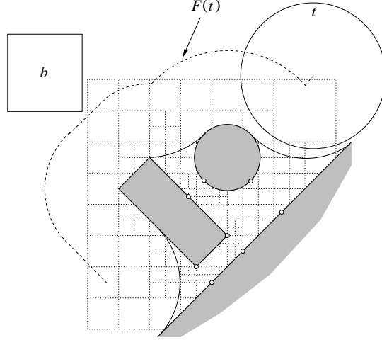
Figure 5: Large-tool BMA for tool t . The solid square is a grid square b in \mathcal{G}_t . The quadtree cells shown in dotted lines are within b \oplus 4t . All of them are small for t and so b induces large tool BMAs of t on them. After these large tool BMAs, some cells will be milled completely and some are milled up to accessibility arcs (shown in solid lines). The boundary of \mathcal{F}(t) is shown in dashed lines.
