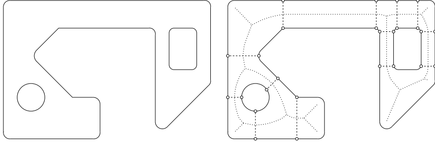
Figure 2: The dotted curve shows the Voronoi diagram of the domain. White points are the bottleneck points and dashed segments are the bottleneck segments.
