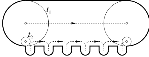
Figure 1: Counterexample for the simplest milling strategy.
