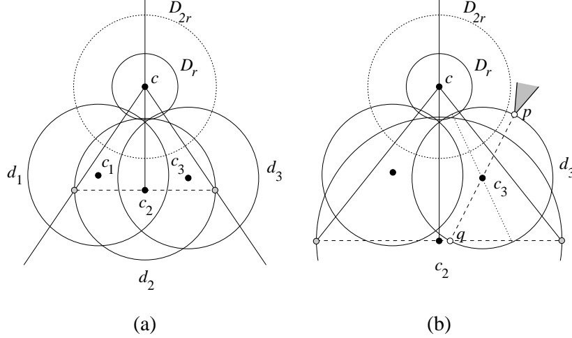
Figure 10: Bounding the combinatorial complexity of unmilled regions for large-tool BMAs.
