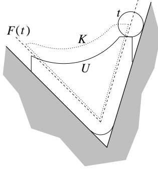
Figure 7: Small-tool BMA. U is bounded by the domain boundary and solid lines. \mathcal{F}(t) is shown with dashed lines, and K is shown with dotted lines. All of U is milled except the portion below the accessibility arc at the bottom.
