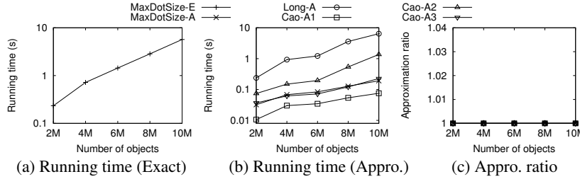
Fig. 5. Scalability test
