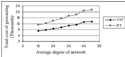
(a) Total cost of geocasting
