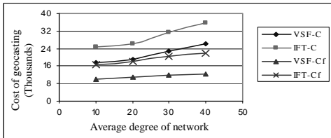
Figure 19 Costs for void networks with 30 voids and 5 \times 2.5 regions
