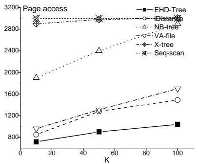
(c). clustered dataset
