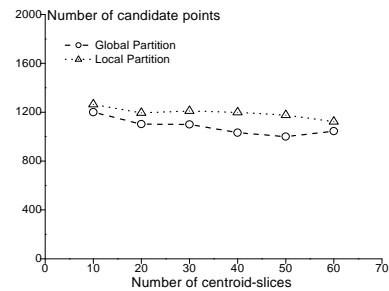
Figure 13. Global Partition vs. Local Partition
