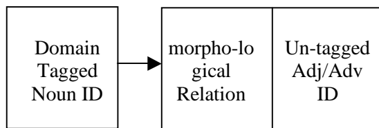
Figure 2. JOIN Method
