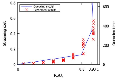
Fig. 3. Streaming cost model at proxy server.
