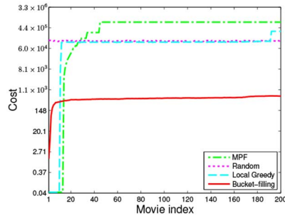
Fig. 11. Cost of each movie given different schemes.
