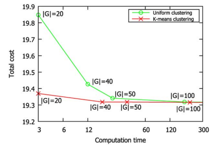
Fig. 14. Total cost versus computation time given different schemes.
