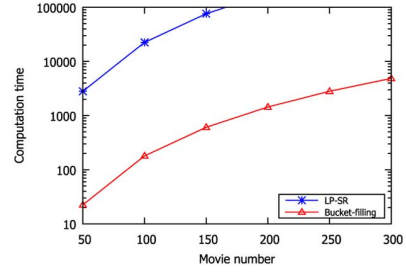
Fig. 8. Computation time versus movie number given different schemes.
