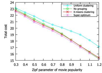
Fig. 12. Total cost versus Zipf parameter of movie popularity given different schemes.
