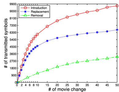
Fig. 15. Number of transmitted symbols versus number of movie change.
