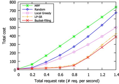
Fig. 7. Total cost versus request rate given different schemes.
