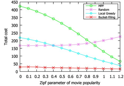
Fig. 9. Total cost versus Zipf parameter of movie popularity given different schemes.
