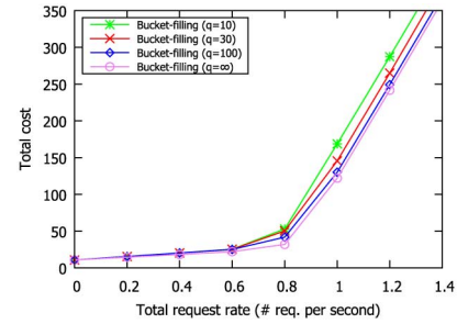
Fig. 4. Total cost versus request rate given q .
