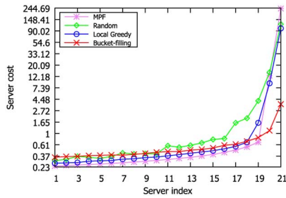
Fig. 10. Server cost distribution given different schemes.
