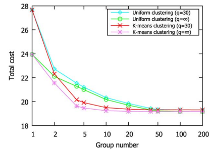
Fig. 13. Total cost versus group number given different schemes.
