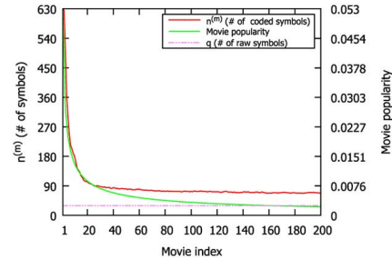
Fig. 5. Optimal n^{(m)} versus movie index.
