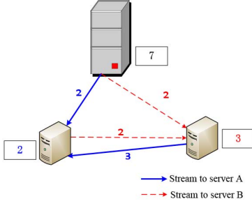
Fig. 2. Illustrative example for bucket-filling with q = 7 , one movie, n^{(1)} = 12 , and two proxy servers.
