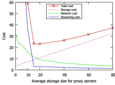
Fig. 6. Total cost and the cost components versus proxy storage.
