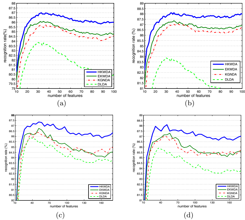
Fig. 1. Comparative performance of HKWDA, EKWDA, KGNDA and DLDA. (a) Polynomial kernel on the mixed data set; (b) RBF kernel on the mixed data set; (c) Polynomial kernel on the subset of FERET; (d) RBF kernel on the subset of FERET.
