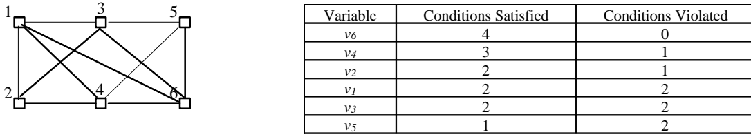
Figure 9: Example of solution splitting during crossover
